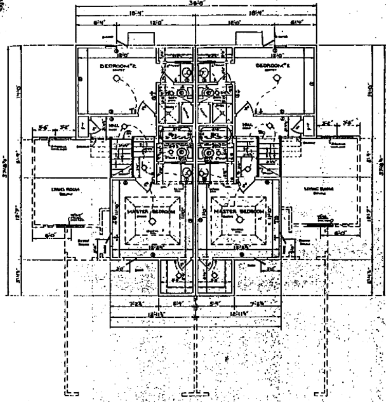
UNIT A BLL A UNIT B BLL B SECOND FLOOR PLAN SCALE 1/4" = 1'-0"
